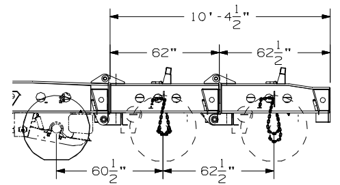
OPTIONAL INTERMEDIATE AND FLIP AXLE
